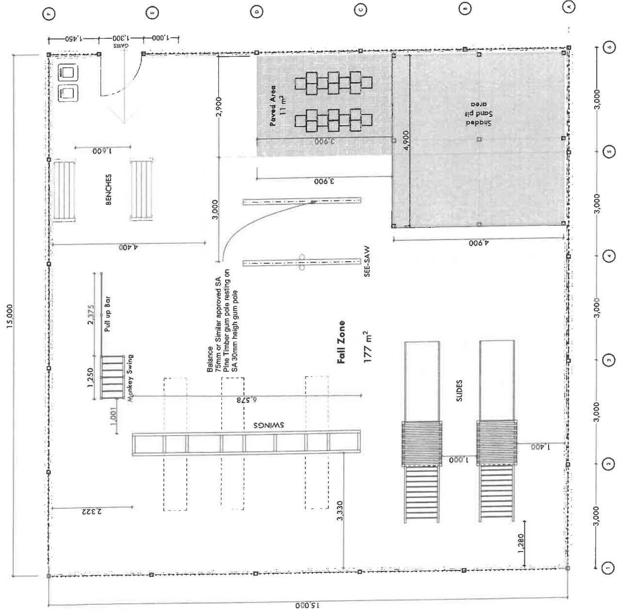
PLAN LAYOUT SCALE 1:75
