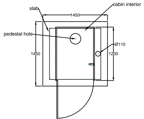
FLOOR ELEVATION SINGLE PIT LATRINE
