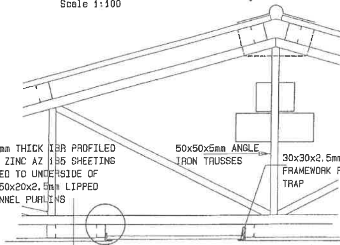
DETAIL A SECTION A
