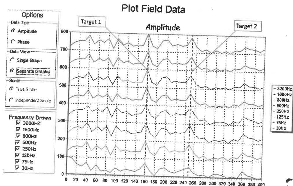
Figure 16: FDEM-8 results for Okatumba west
