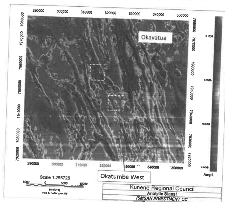
Figure 14: Analytic Signal map at Okavatus and Okatumba west, Opuwo rural
