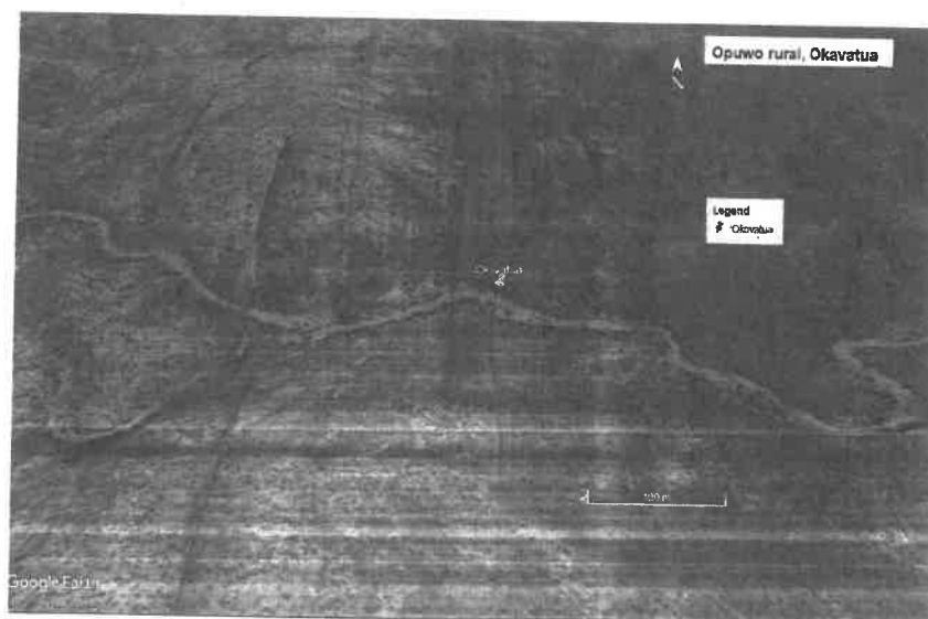
Figure 18: Okovatua mapped base on lineaments (red lines) due to terrain
