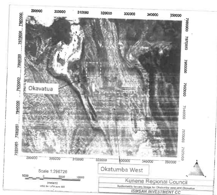
Figure 15: Radiometric data for Okatumba west and Okavatus, Opuwo rural
