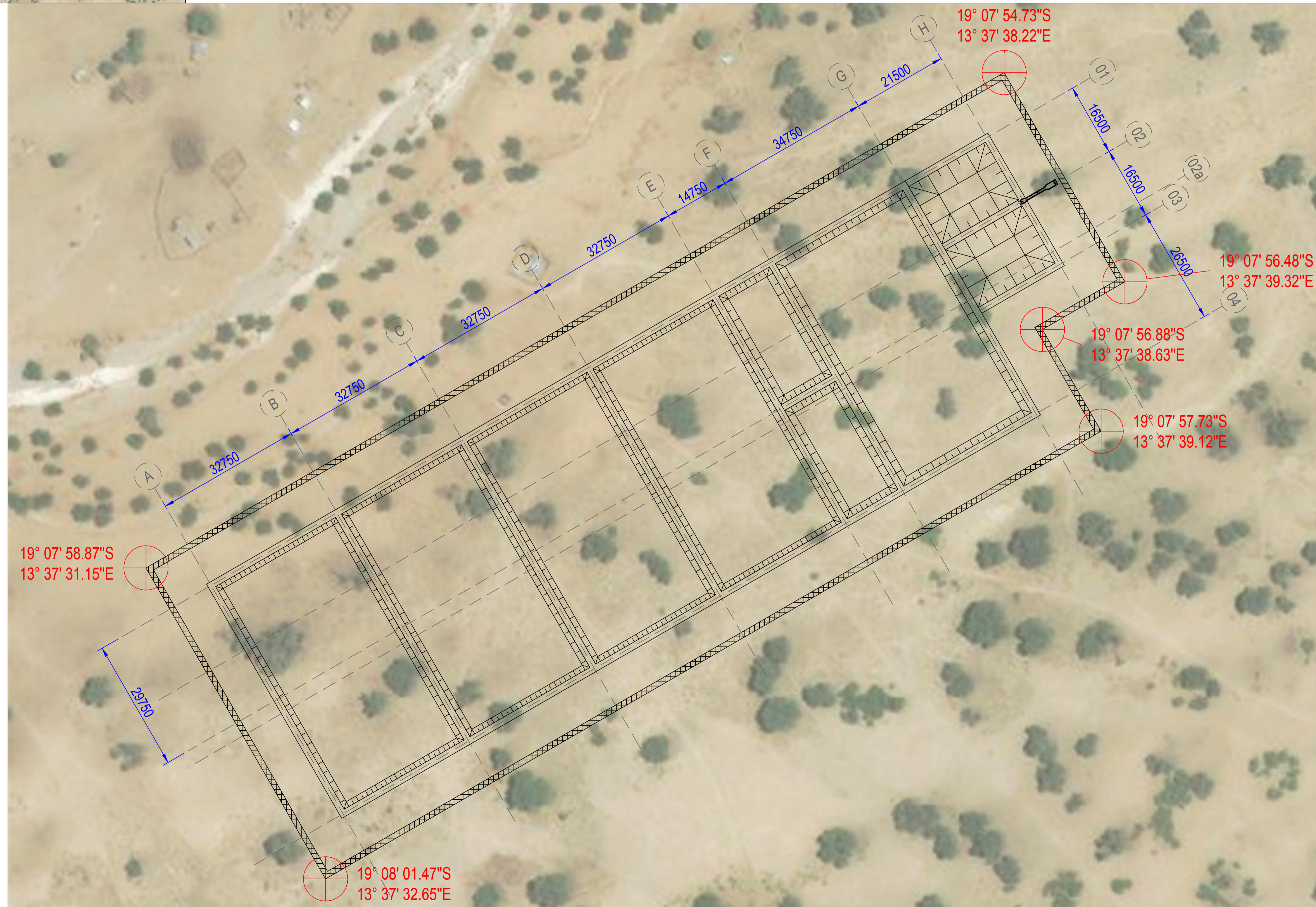
OXIDATION POND LAYOUT & FENCE SETTING OUT
